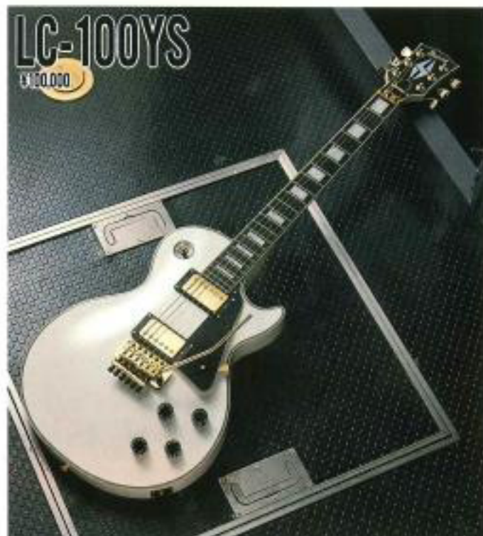
LC-100YS ¥180,000 NECK/Mahogany FINGER BOARD/Rosewood, 22F, 250R, 24.75" Scale NECK JOINT/Set Neck BODY/Maple-Top, Mahogany-Back PICKUP/VH-3 CONTROL/2V, 2T, Toggle SW. BRIDGE/FRT-4G COLOR/H
