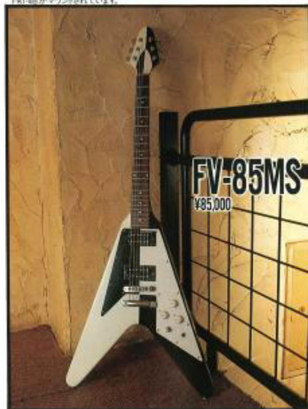
FV-85MS ¥85,000 NECK/Mahogany FINGER BOARD/Rosewood, 22F, 250R, 24.75" Scale NECK JOINT/Set Neck BODY/Mahogany PICKUP/VH-2 CONTROL/2V, 1T, Toggle SW BRIDGE/Tune O Matic, Stop Tailpiece-Cr COLOR/H-BL Combination
