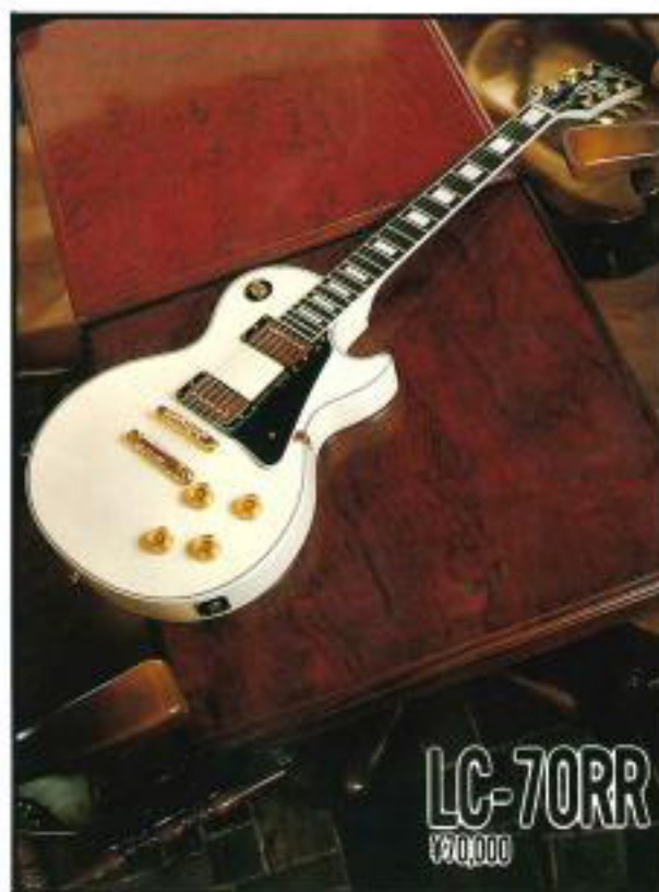
NECK/Mahogany FINGER BOARD/Rosewood, 22F, 250R, 24.75" Scale NECK JOINT/Set Neck BODY/Maple-Top, Mahogany-Back PICKUP/VH-3 CONTROL/2V, 2T, Toggle SW. BRIDGE/Tune O Matic, Stop Tailpiece-G COLOR/CH
