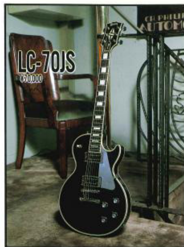
NECK/Mahogany FINGER BOARD/Rosewood, 22F, 250R, 24.75" Scale NECK JOINT/Set Neck BODY/Maple-Top, Mahogany-Back PICKUP/VH-3 (front), VH-3 (rear) CONTROL/2V, 2T, Toggle SW. BRIDGE/Tune O Matic, Stop Tailpiece-Cr COLOR/BL
