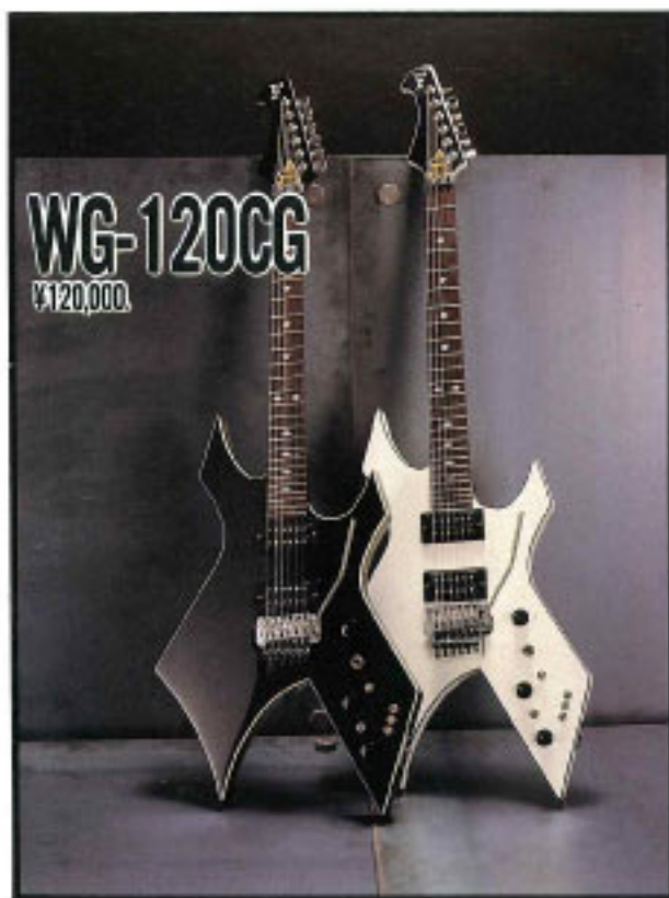
WG-120CG ¥120,000 NECK/Maple FINGER BOARD/Rosewood, 24F, 350R, 24.75" Scale NECK JOINT/Neck Through Body BODY/Mahogany PICKUP/VH-4 CONTROL/1V, 1T, Bst-V, Toggle SW, Mini SW BRIDGE/HEAD CRASHER FRT-5C COLOR/BL, H
