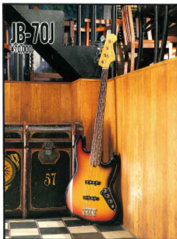
NECK/Maple FINGER BOARD/Rosewood, Fretless, 170R, 34.00"Scale NECK JOINT/Detachable BODY/Alder PICKUP/VJB-1N(front), VJB-1B(rear) CONTROL/2V, 1T BRIDGE/Combination, Cr COLOR/Y90
